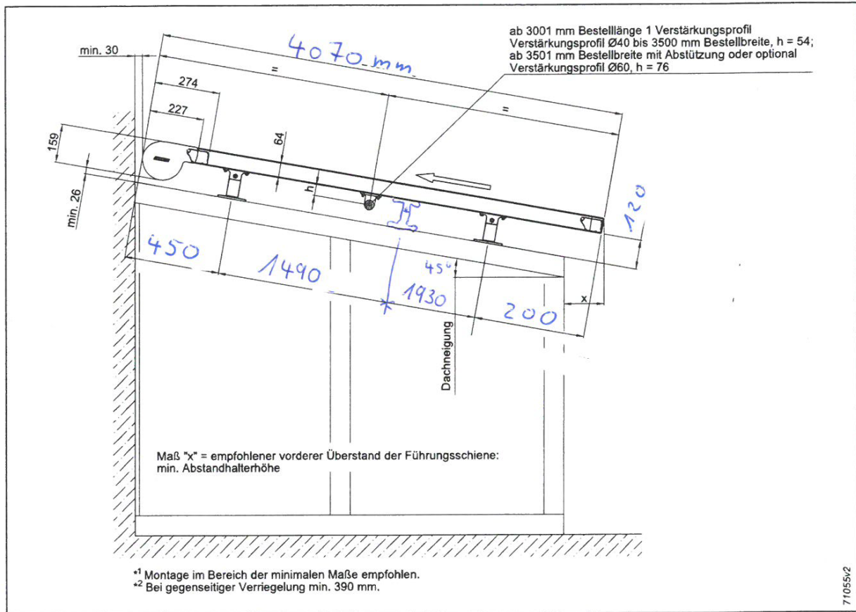
Abb. 330: Wintergarten-Markise W19
