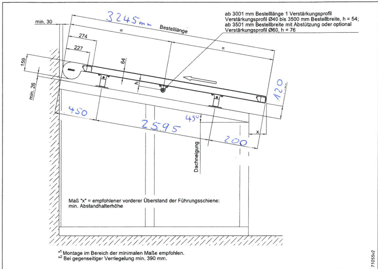
Abb. 330: Wintergarten-Markise W19
