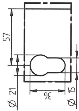
Detail A
